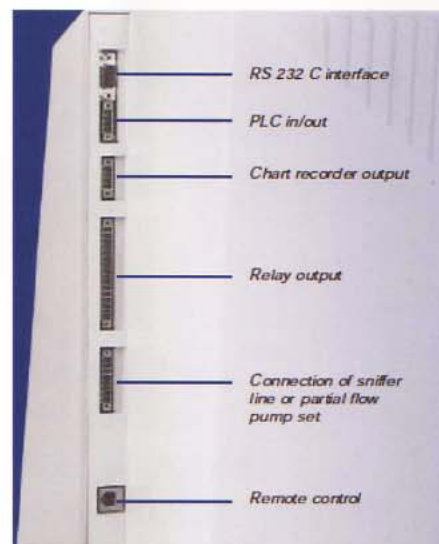
Electrical connection strip on the rear
